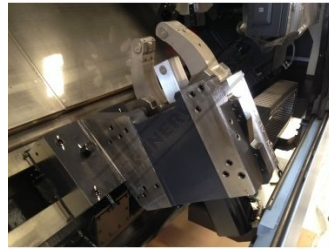
Hydraulic Steady
