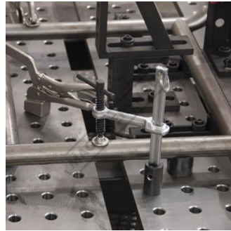
Used in Combination with a Straight Edge Stop and V Block to Hold a Round Tube
