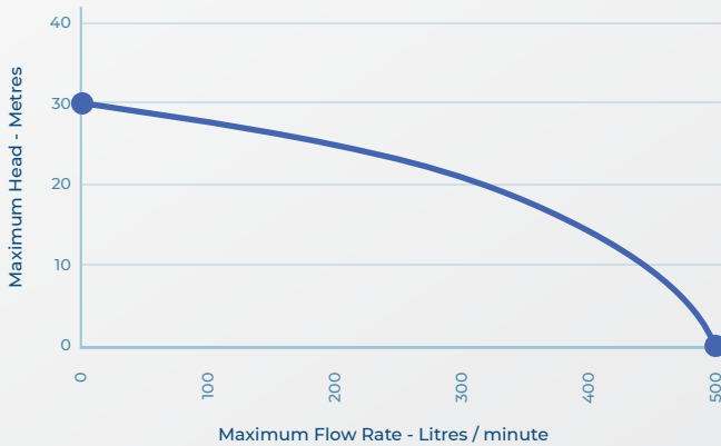
MY20 PUMP PERFORMANCE CURVE
